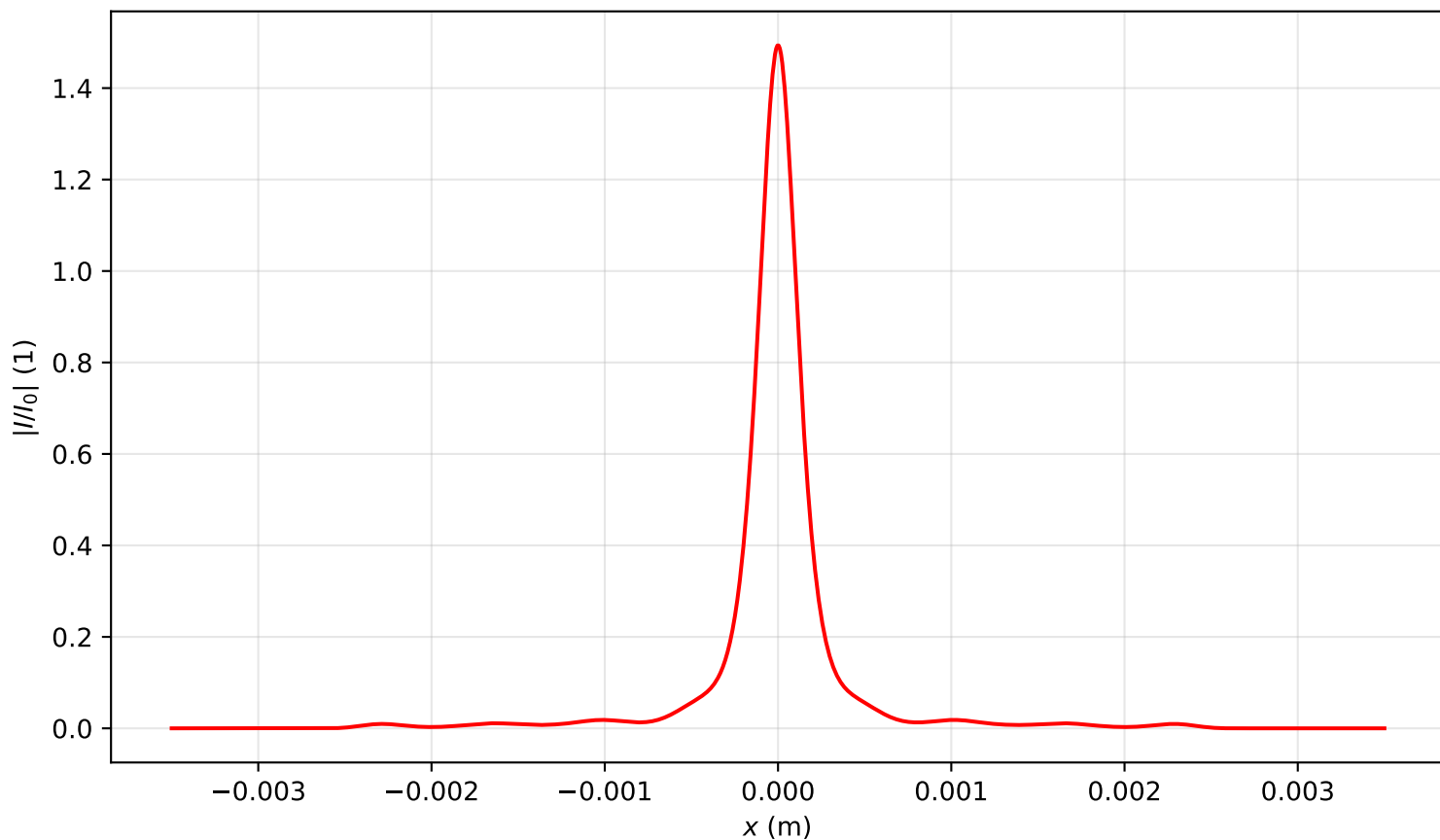
Intensity profile I(x, y = 0, z = 3.981)/I_0 , P_{in}=3.0P_{cr} , artificial time
